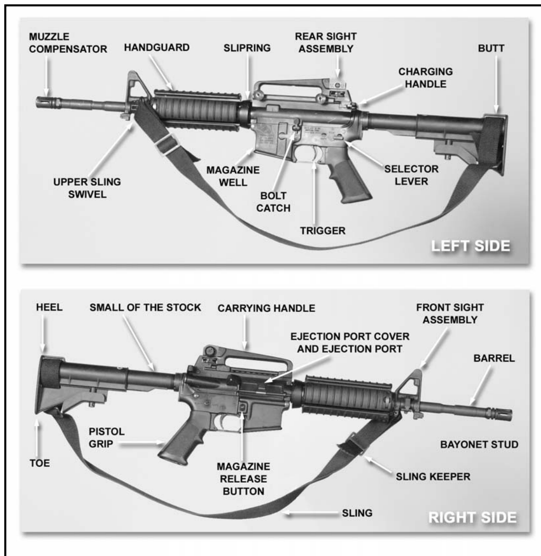
Figure B-1. Nomenclature, M4-series carbine.
